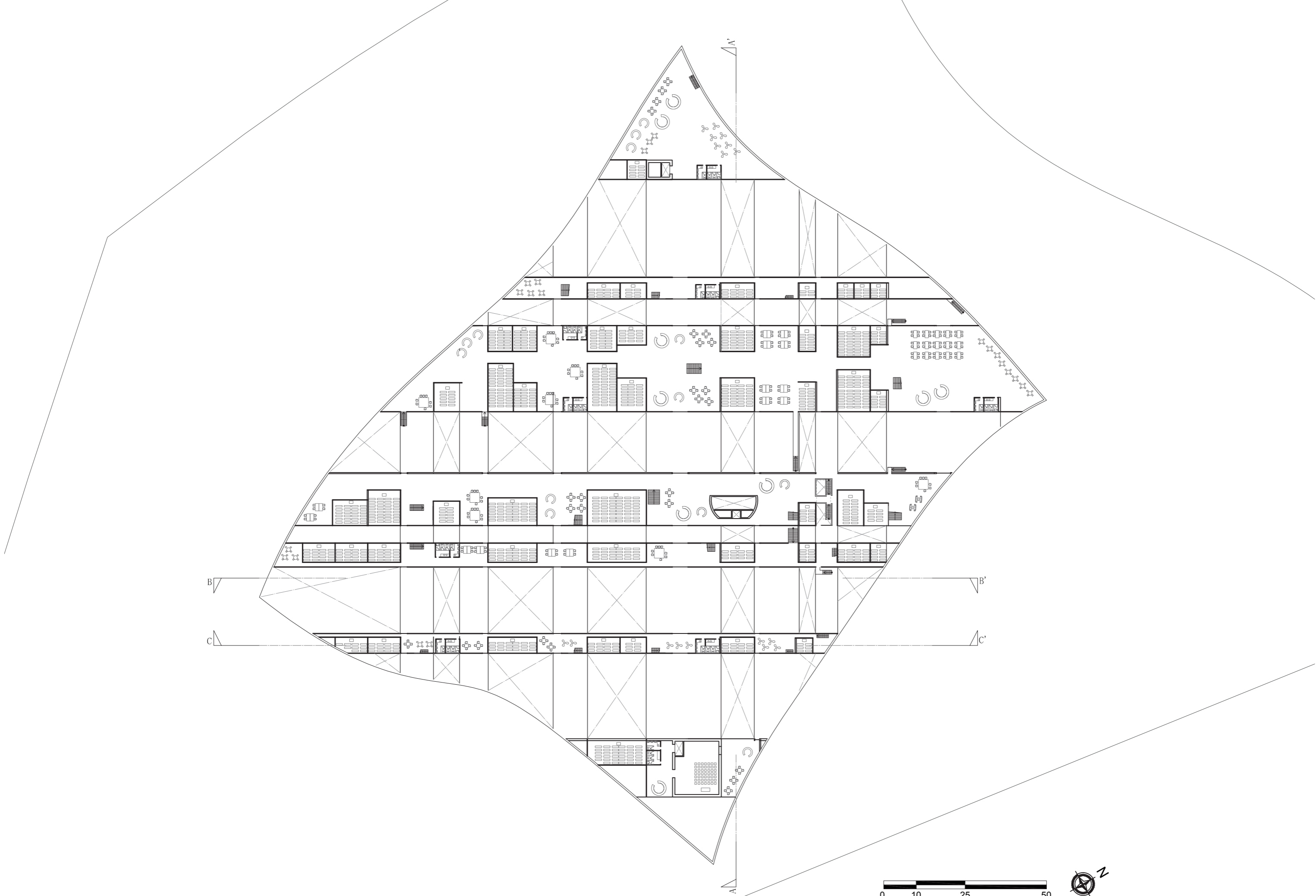
2F Drawing
